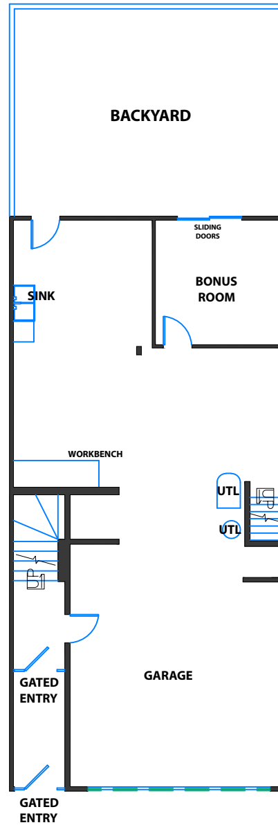
LOWER LEVEL
