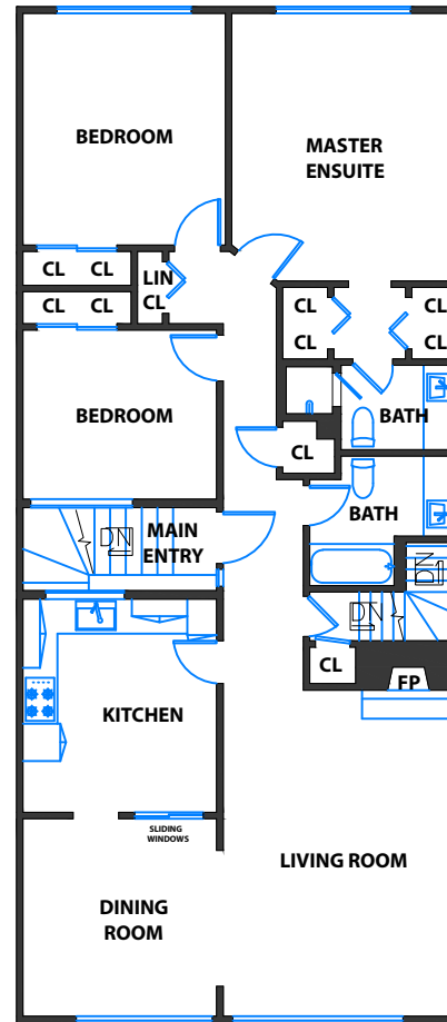
MAIN LEVEL
